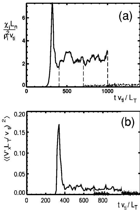
FIG. 6. Time histories of (a) \chi_i and (b) the mean squared \mathbf{E} \times \mathbf{B} shearing rate (L_{Ti} S / v_{ii})^2 associated with the flux-surface-averaged electrostatic potential, both in the absence of scrambling and when restarts with scrambling and gradient reduction are done at three times during the run. Cyclone DIII-D base-case parameters were used.
